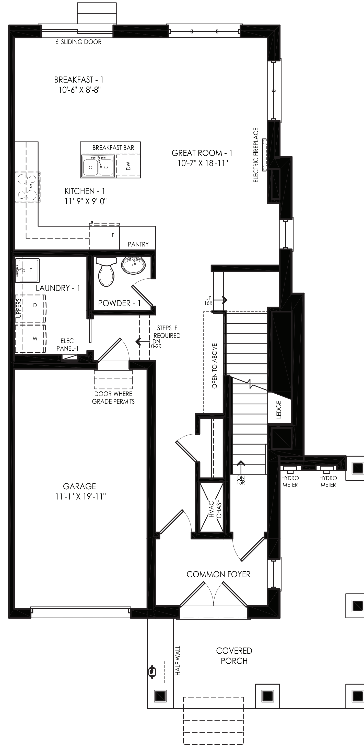
GROUND FLOOR
