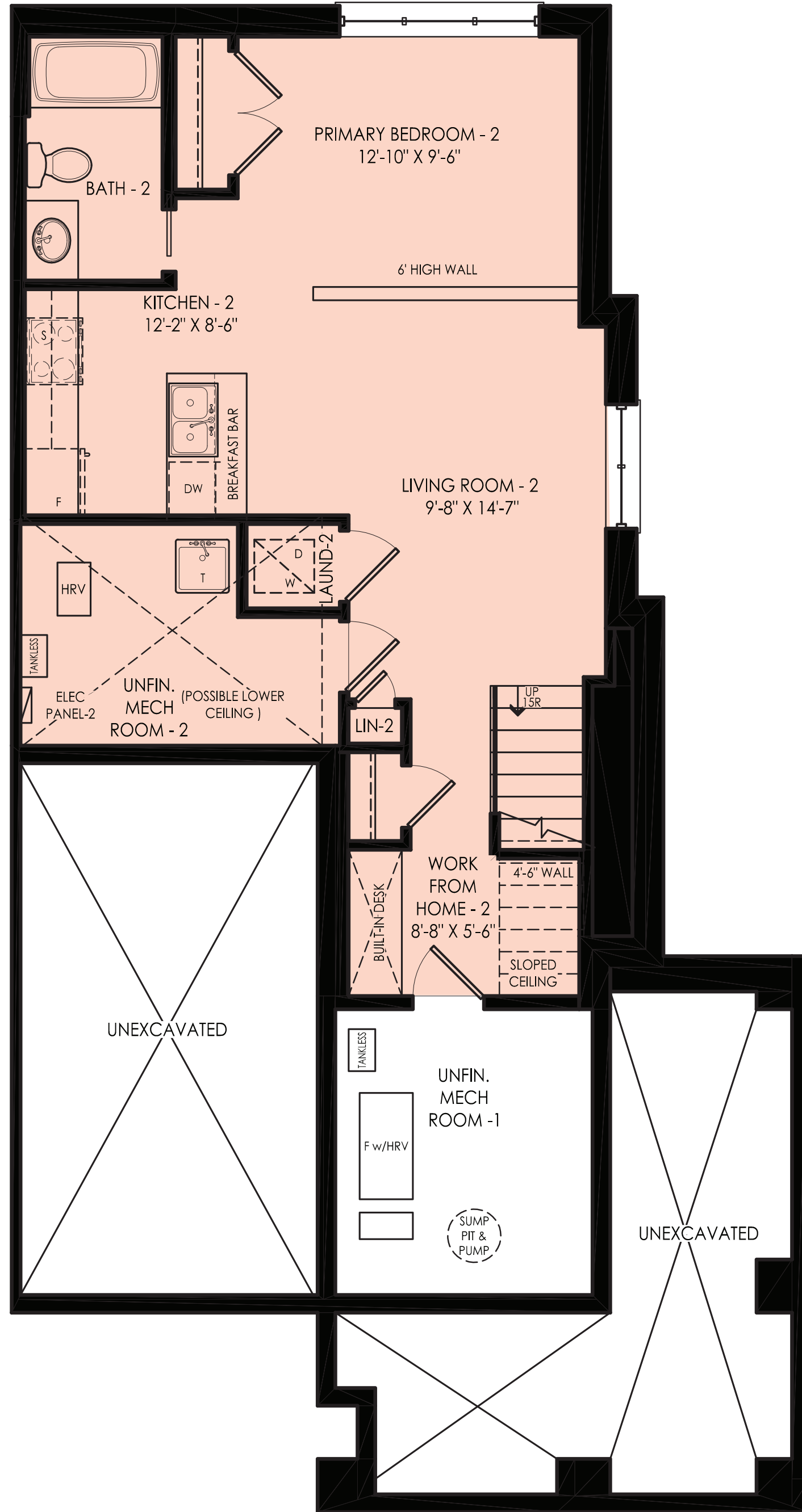
BASEMENT FLOOR PLAN WITH SECONDARY DWELLING UNIT
